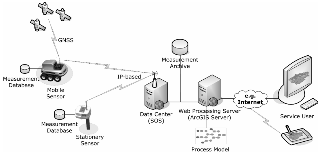
Figure 2: Real-time Situational Awareness Topology.
